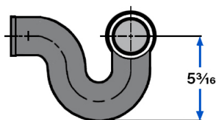
9-344 (LEFT HAND)
