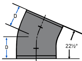
SIXTEENTH BEND
