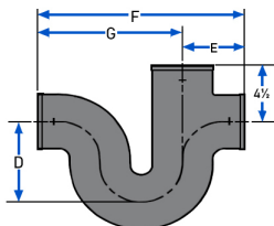
RUNNING TRAP w/4" SINGLE VENT
