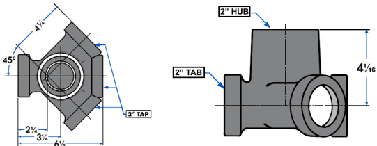
2" Tapped Double Wye w/2" Hub Vent
