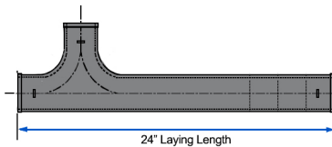
Double Sweep San Tee
